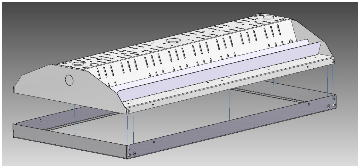
Figure 1: Slide assembled frame onto fixture
