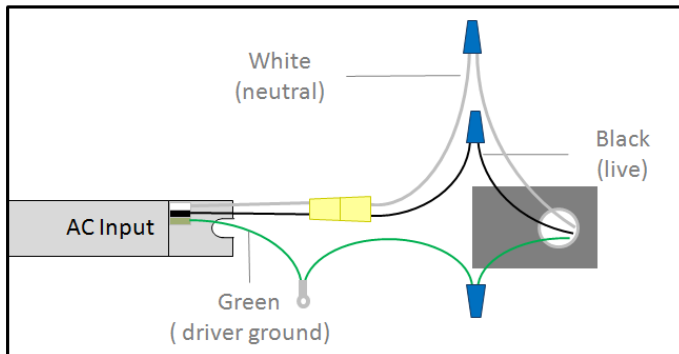
Diagram C: Magnified AC Connection Diagram
