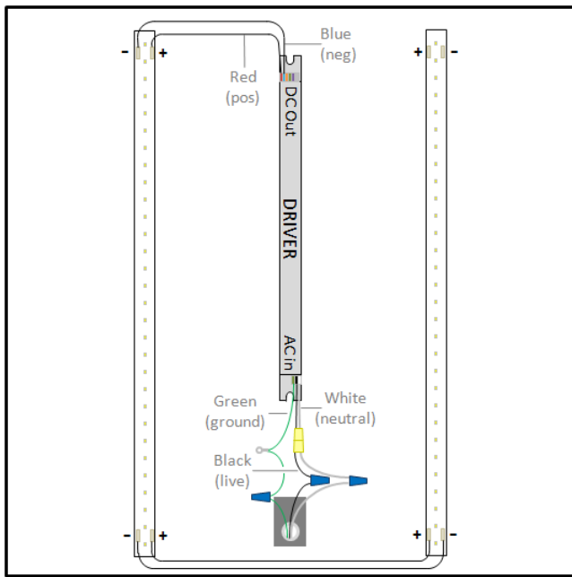
Diagram A: 2' x 2' Troffer Layout and Wiring: Mount LED boards approximately 5" from the fixture center.
