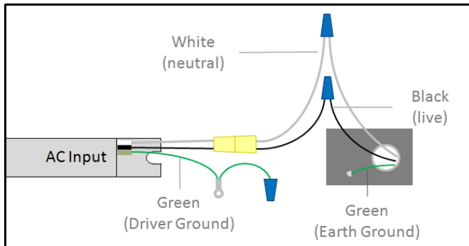
Diagram A: 2' x 2' Troffer Layout and Wiring: Mount LED boards approximately 5" from the fixture center.
