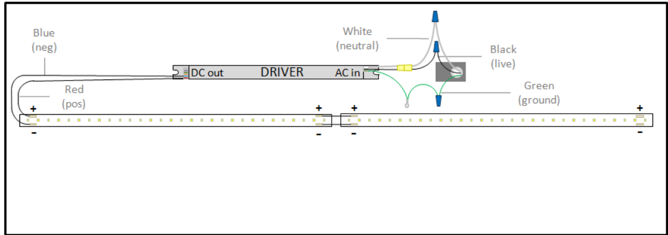
Diagram B: 1' x 4' Troffer Layout and Wiring: Mount LED boards along the fixture center. In some fixtures it may be necessary to mount the LED boards onto the fluorescent ballast cover.
