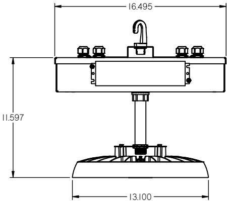
EM/W Housing
