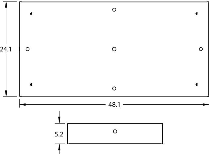
2x4 Surface Mount Dimensions
