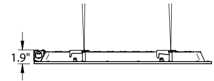
Suspended
